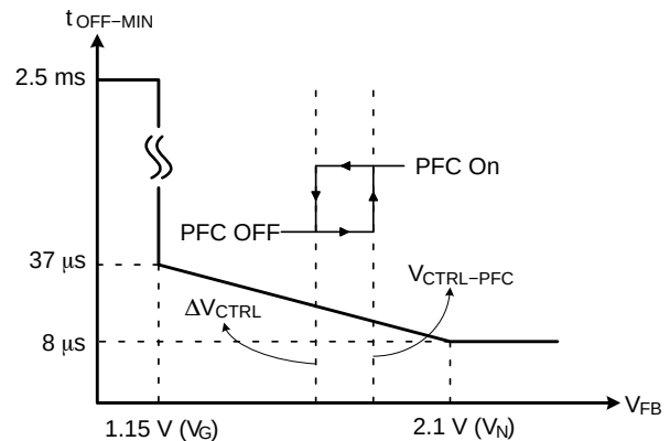
Figure 37. V_{FB} Voltage vs. t_{OFF-MIN} Time Characteristic Curve
