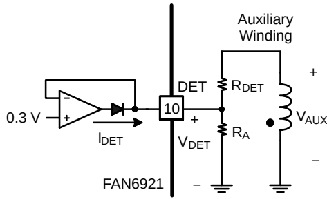
Figure 38. Valley Detection
