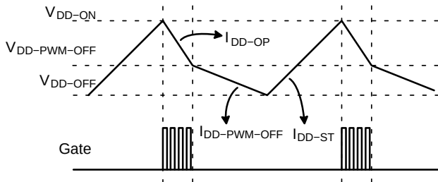
Figure 36. Typical Waveform of V_{DD} Voltage and Gate Signal at Hiccup Mode Operation
