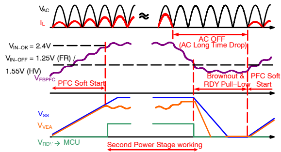
Figure 26. When AC Drops for a Long Time
