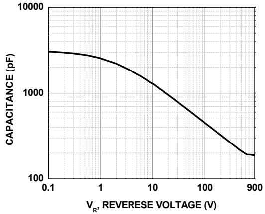
Figure 6. Capacitive vs. Reverse Voltage
