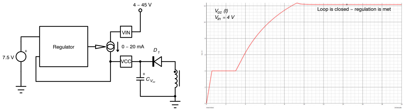
Figure 35. The LDO Can Be Associated with an Auxiliary Winding and Be Turned Off in Normal Operation
