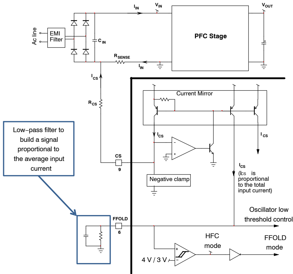
Figure 17. Frequency Foldback Control
