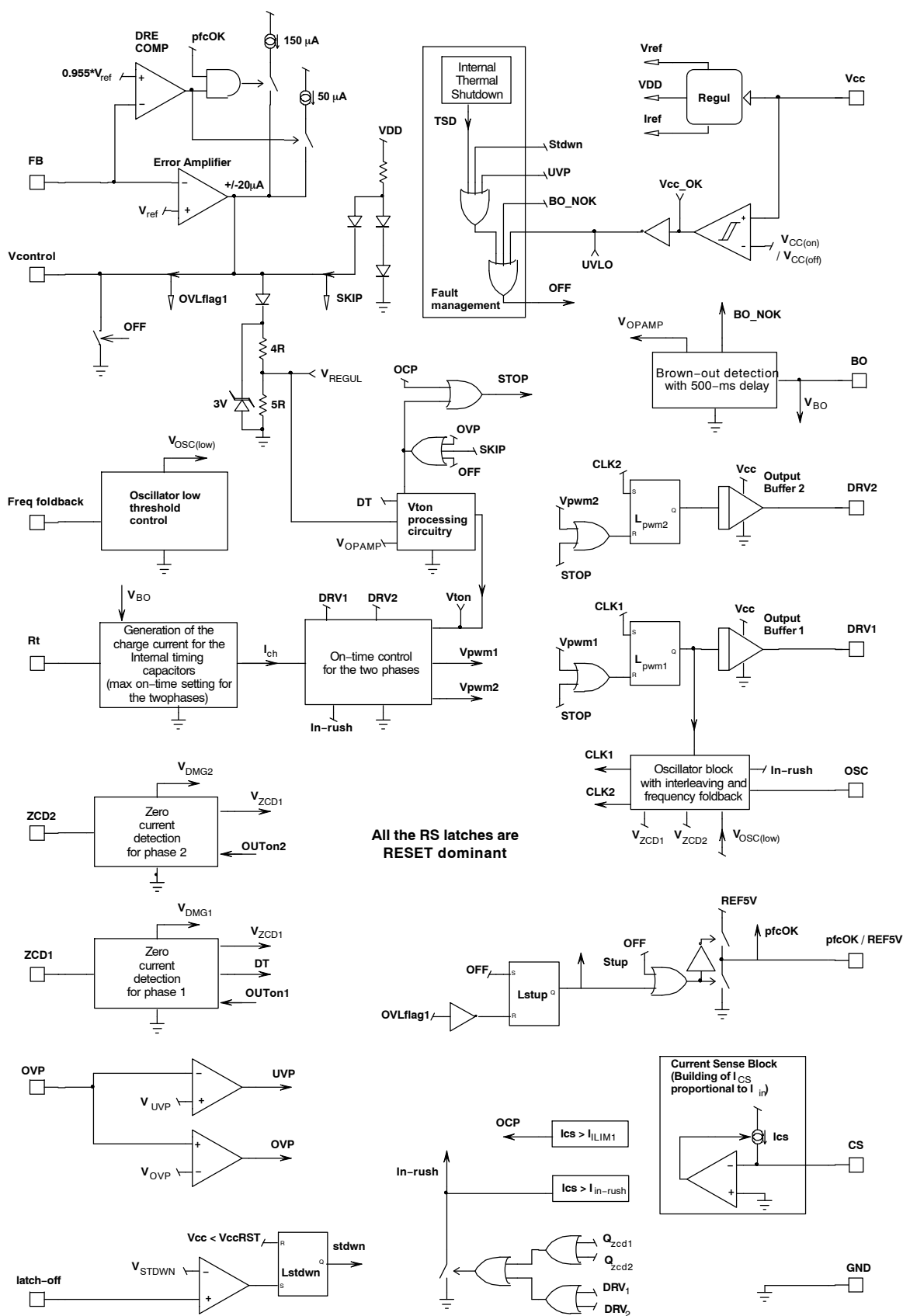
Figure 2. Block Diagram
