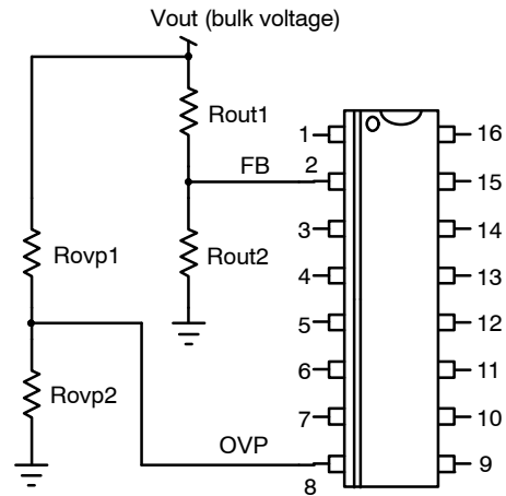
Figure 12. Configuration with Two Separate Feed-back Networks
