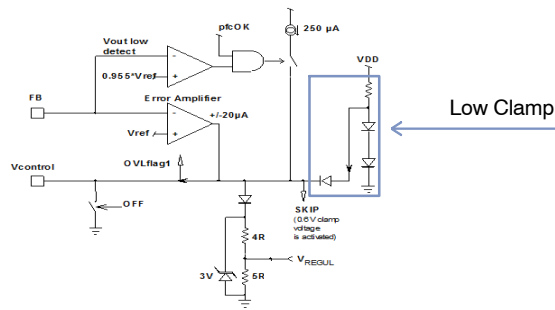
Figure 20. V_{CONTROL} Low Clamp
