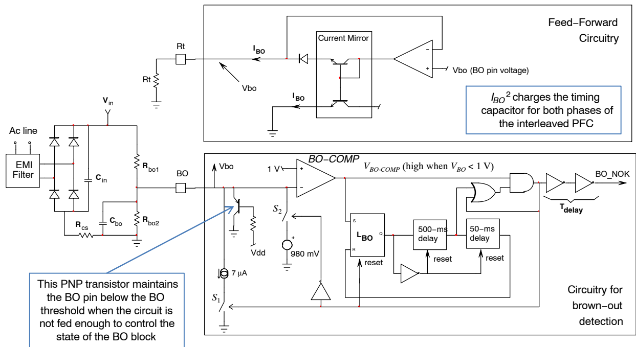
Figure 21. Brown-out Block
