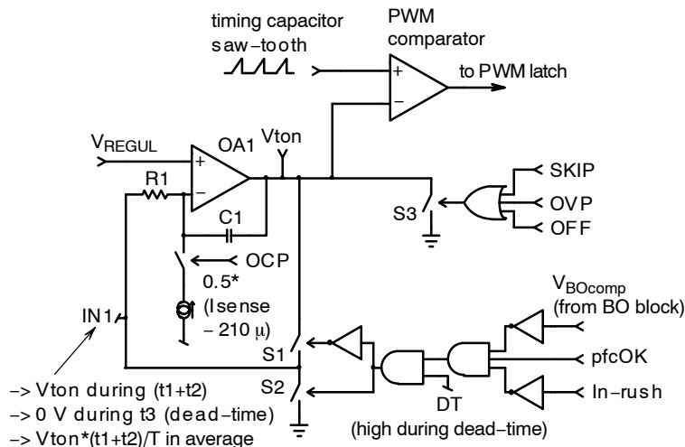
Figure 5. V_{\text{ton}} Processing Circuit
