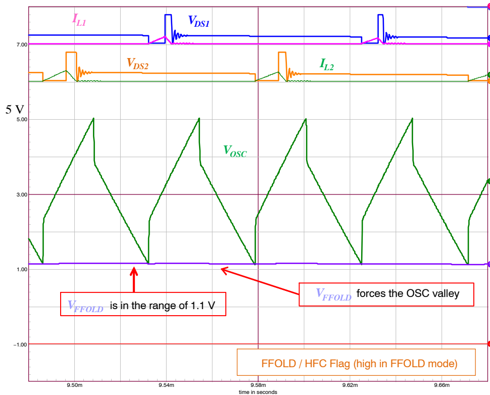
Figure 16. Operation at a Low V_{FFOLD} Value ( V_{FFOLD} = 1.1\text{ V} )
