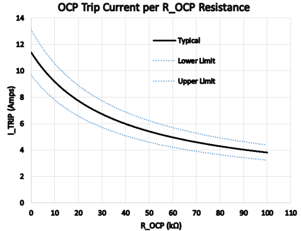
Figure 25. OCP Trip Current Setting
