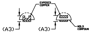
DETAIL B ALTERNATE CONSTRUCTIONS
