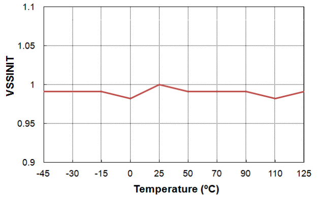
Figure 34. VSS.INIT vs. Temperature
