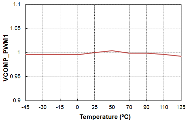
Figure 23. VCOMP.PWM vs. Temperature
