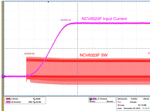
Figure 46. Inrush Current ( V_{IN} = 3.3\text{ V} , V_{OUT} = 1.8\text{ V} , I_{OUT} = 800\text{ mA} , C_{OUT} = \text{GCM21BR70J106KE22} , L = \text{FSD0420-H-1R0M} )
