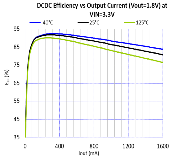
Figure 15. Efficiency vs. Output Current and Temperature at V_{IN} = 3.3\text{ V} ( V_{OUT} = 1.8\text{ V} , L = \text{FDSD0420-H-1R0M} )
