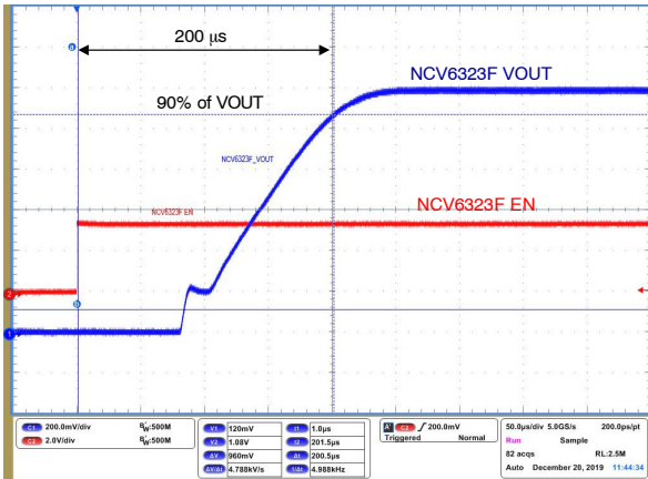
Figure 48. Startup Time T_{START} (NCV6323FCLMTW12, C_{OUT} = 10\text{ }\mu\text{F} )
