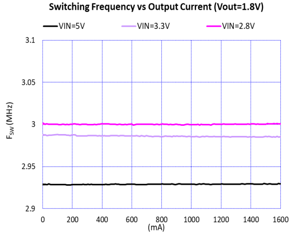
Figure 29. Switching Frequency vs Output Current ( V_{OUT} = 1.8\text{ V} , T_A = 25^\circ\text{C} )
