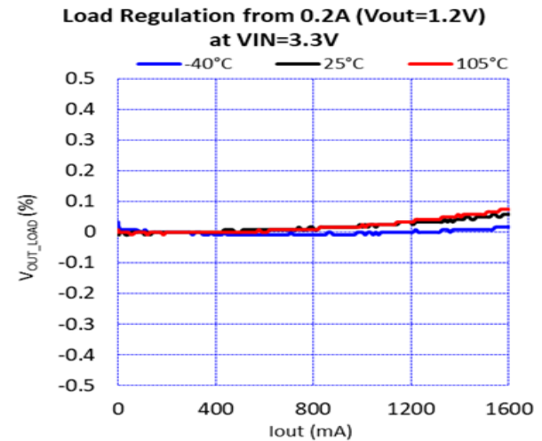
Figure 21. Load Regulation ( V_{IN} = 3.3\text{ V} , V_{OUT} = 1.2\text{ V} )
