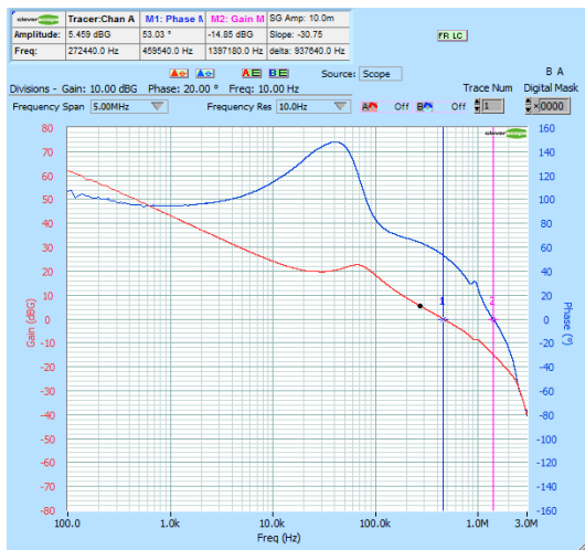
Figure 62. Bode Plot NCV6323FxLMTW10TBG L = 1.0 μH – COUT = 10 μF
