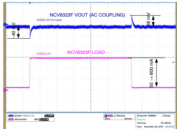
Figure 33. Load Transient ( V_{IN} = 3.3\text{ V} , V_{OUT} = 1.2\text{ V} , C_{OUT} = \text{GCM21BR70J106KE22} , L = \text{FDSD0420-H-1R0M} ) 50 mA \rightarrow 600 mA \rightarrow 50 mA
