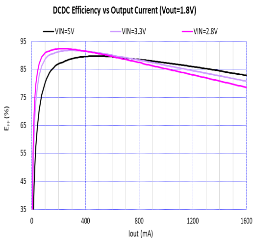
Figure 14. Efficiency vs. Output Current and Input Voltage ( V_{OUT} = 1.8\text{ V} , T_A = 25^\circ\text{C} , L = \text{FDSD0420-H-1R0M} )
