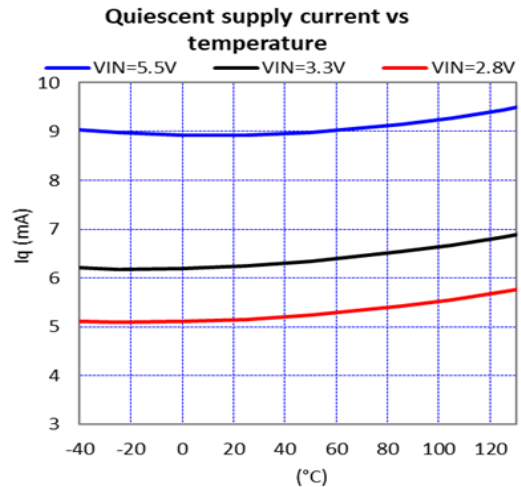
Figure 9. Quiescent Current vs. Temperature (EN = High, V OUT = 1.8 V, No Load)
