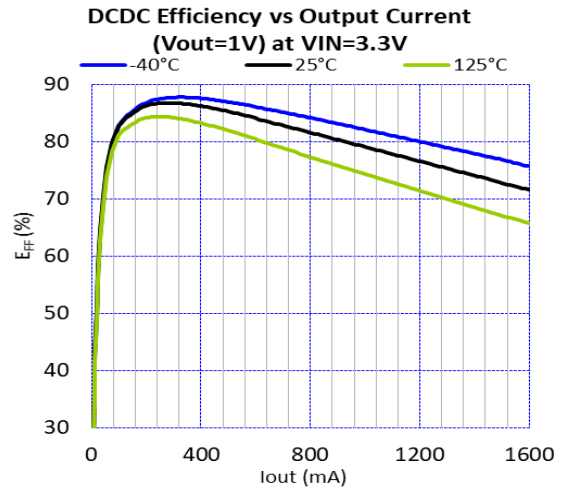
Figure 11. Efficiency vs. Output Current and Temperature at V_{IN} = 3.3\text{ V} ( V_{OUT} = 1.0\text{ V} , L = \text{FDSD0420-H-1R0M} )
