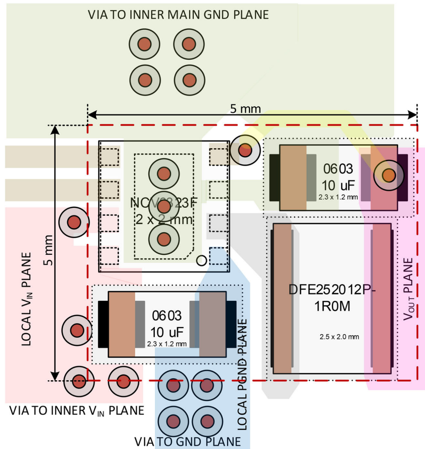
Figure 67. Recommended Minimal Size PCB Layout (Without Optional C_{AVIN} )
