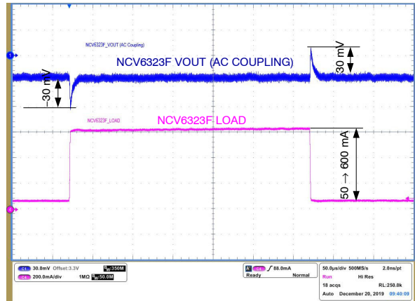
Figure 37. Load Transient ( V_{IN} = 5.0\text{ V} , V_{OUT} = 3.3\text{ V} , C_{OUT} = \text{GCM21BR70J106KE22} , L = \text{FDSD0420-H-1R0M} ) 50 mA \rightarrow 600 mA \rightarrow 50 mA
