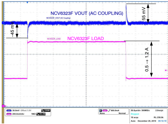
Figure 30. Load Transient ( V_{IN} = 3.3\text{ V} , V_{OUT} = 1.0\text{ V} , C_{OUT} = \text{GCM21BR70J106KE22} , L = \text{FDSD0420-H-1R0M} ) 500 mA \rightarrow 1.2 A \rightarrow 500 mA
