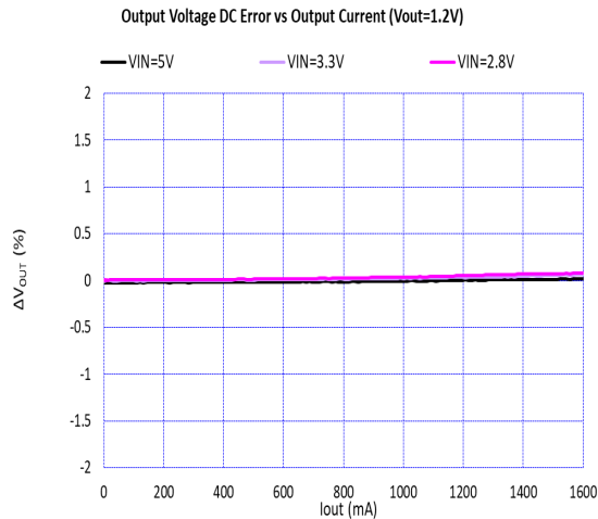
Figure 26. Output Voltage DC Error vs Output Current ( V_{OUT} = 1.2\text{ V} , T_A = 25^\circ\text{C} )
