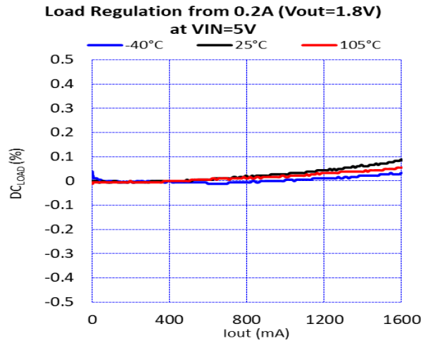
Figure 23. Load Regulation ( V_{IN} = 5.0\text{ V} , V_{OUT} = 1.8\text{ V} )
