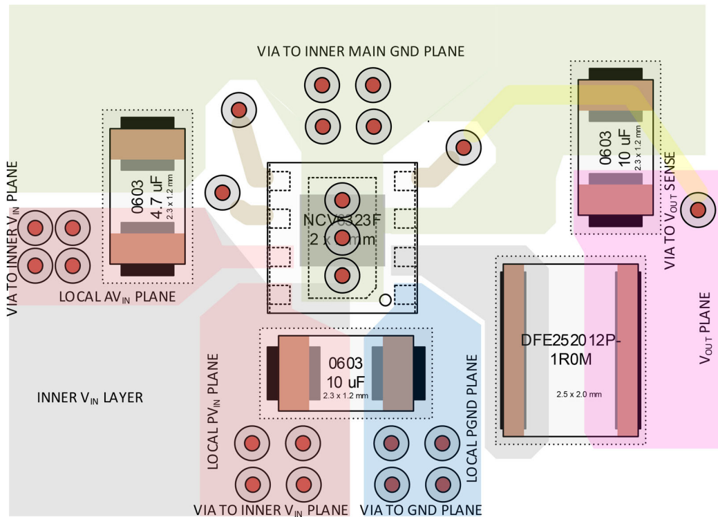
Figure 68. Recommended Large Size PCB Layout (With Optional C_{AVIN} )
