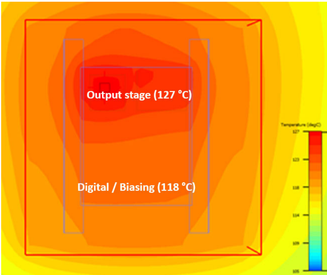
Figure 65. Die Temperature Simulation (500 mW Dissipated Power)
