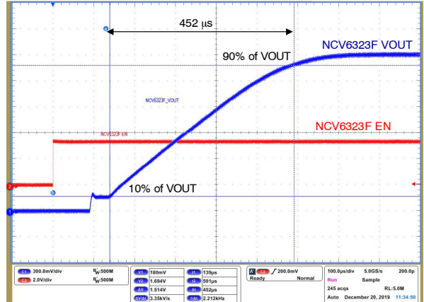
Figure 53. Soft Start Time T_{SS} (NCV6323FELMTW18, C_{OUT} = 10 \mu F )
