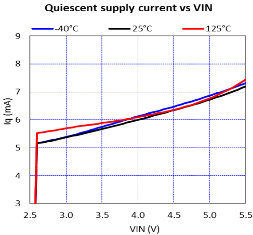
Figure 6. Quiescent Current vs. Input Voltage (EN = High, V OUT = 1.2 V, No Load)
