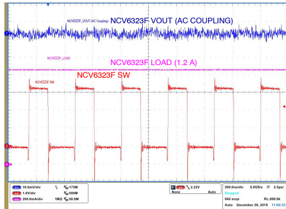
Figure 43. Output Voltage Ripple ( V_{IN} = 3.3\text{ V} , V_{OUT} = 1.2\text{ V} , C_{OUT} = \text{GCM21BR70J106KE22} , I_{OUT} = 500\text{ mA} )
