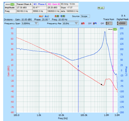
Figure 63. Bode Plot NCV6323FxLMTW10TBG L = 1.0 μH – COUT = 100 μF
