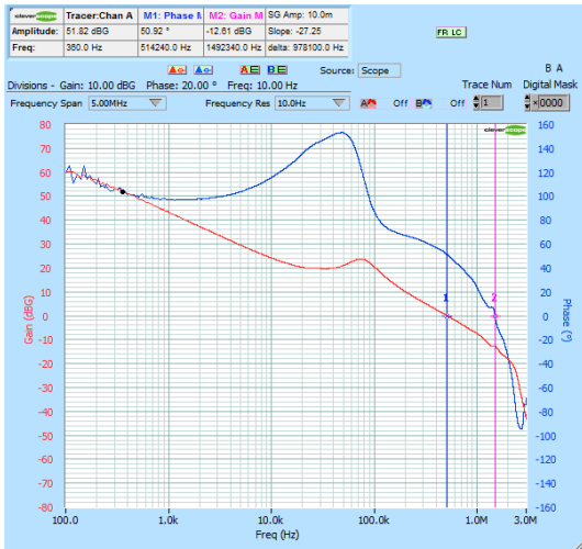
Figure 58. Bode Plot NCV6323FxLMTW33TBG L = 1.0 μH – COUT = 10 μF
