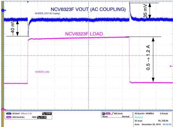
Figure 36. Load Transient ( V_{IN} = 5.0\text{ V} , V_{OUT} = 3.3\text{ V} , C_{OUT} = \text{GCM21BR70J106KE22} , L = \text{FDSD0420-H-1R0M} ) 500 mA \rightarrow 1.2 A \rightarrow 500 mA
