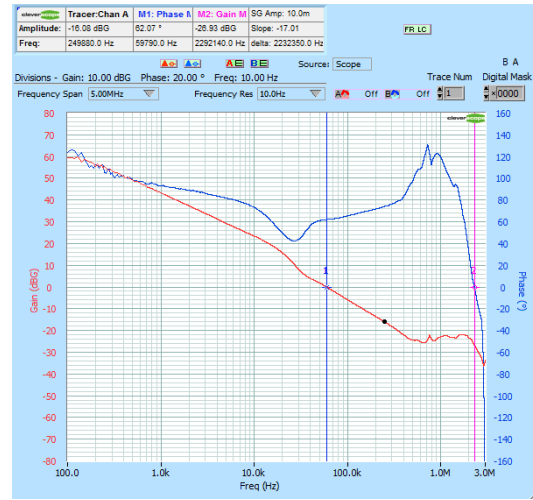
Figure 59. Bode Plot NCV6323FxLMTW33TBG L = 1.0 μH – COUT = 100 μF
