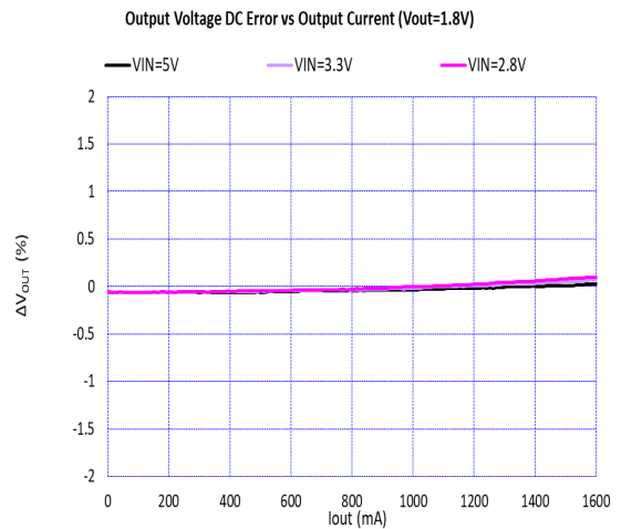
Figure 27. Output Voltage DC Error vs Output Current ( V_{OUT} = 1.8\text{ V} , T_A = 25^\circ\text{C} )
