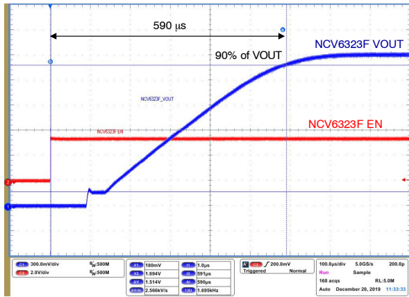
Figure 52. Startup Time T_{START} (NCV6323FELMTW18, C_{OUT} = 10 \mu F )
