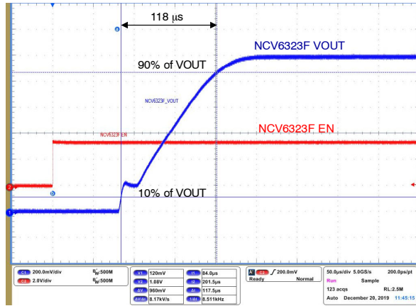
Figure 49. Soft Start Time T_{SS} (NCV6323FCLMTW12, C_{OUT} = 10\text{ }\mu\text{F} )
