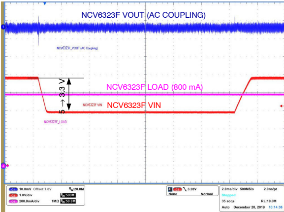
Figure 40. Line Transient ( V_{OUT} = 1.8\text{ V} , C_{OUT} = \text{GCM21BR70J106KE22} , L = \text{FDSD0420-H-1R0M} )
