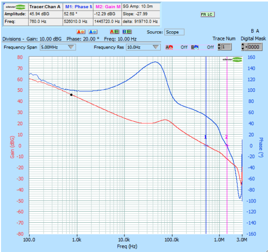
Figure 60. Bode Plot NCV6323FxLMTW12TBG L = 1.0 μH – COUT = 10 μF
