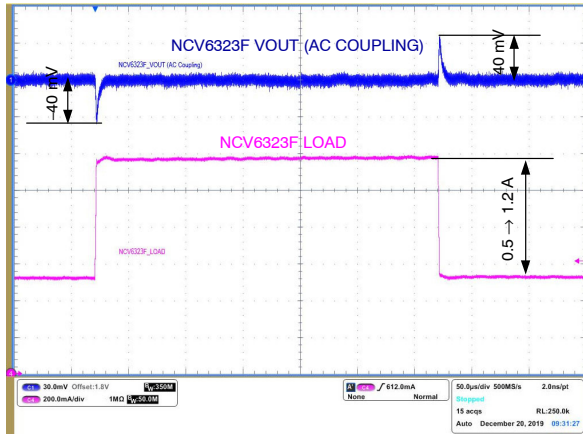
Figure 34. Load Transient ( V_{IN} = 3.3\text{ V} , V_{OUT} = 1.8\text{ V} , C_{OUT} = \text{GCM21BR70J106KE22} , L = \text{FDSD0420-H-1R0M} ) 500 mA \rightarrow 1.2 A \rightarrow 500 mA
