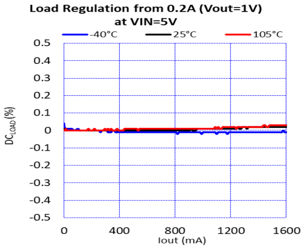
Figure 18. Load Regulation ( V_{IN} = 5.0\text{ V} , V_{OUT} = 1.0\text{ V} )
