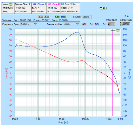
Figure 56. Bode Plot NCV6323FxLMTW18TBG L = 1.0 \mu H - C_{OUT} = 10 \mu F
