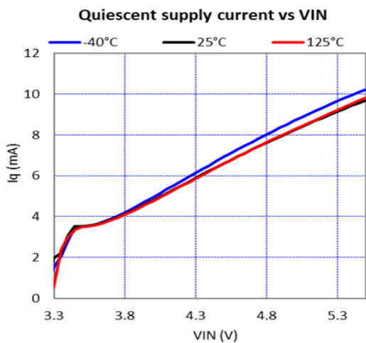
Figure 8. Quiescent Current vs. Input Voltage (EN = High, V OUT = 3.3 V, No Load)
