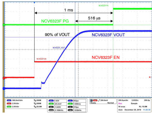
Figure 47. PG Delay after Start Up – NCV6323F-E ( V_{IN} = 3.3\text{ V} , V_{OUT} = 1.8\text{ V} , C_{OUT} = \text{GCM21BR70J106KE22} , L = \text{FSD0420-H-1R0M} )
