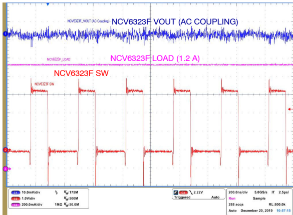
Figure 42. Output Voltage Ripple ( V_{IN} = 3.3\text{ V} , V_{OUT} = 1.0\text{ V} , C_{OUT} = \text{GCM21BR70J106KE22} , I_{OUT} = 500\text{ mA} )
