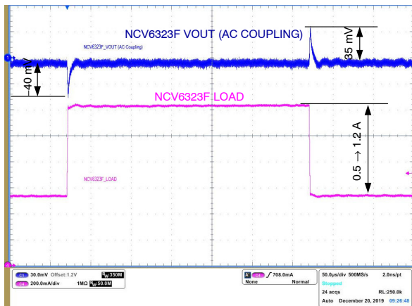
Figure 32. Load Transient ( V_{IN} = 3.3\text{ V} , V_{OUT} = 1.2\text{ V} , C_{OUT} = \text{GCM21BR70J106KE22} , L = \text{FDSD0420-H-1R0M} ) 500 mA \rightarrow 1.2 A \rightarrow 500 mA
