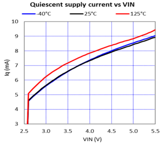
Figure 7. Quiescent Current vs. Input Voltage (EN = High, V OUT = 1.8 V, No Load)
