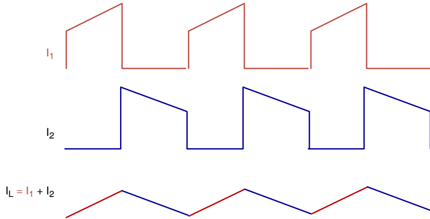
Figure 66. AC Current Flowing Loops
