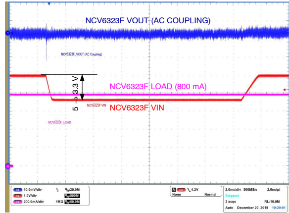
Figure 41. Line Transient ( V_{OUT} = 3.3\text{ V} , C_{OUT} = \text{GCM21BR70J106KE22} , L = \text{FDSD0420-H-1R0M} )
