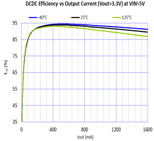
Figure 17. Efficiency vs. Output Current and Temperature at V_{IN} = 5.0\text{ V} ( V_{OUT} = 3.3\text{ V} , L = \text{FSD0420-H-1R0M} )
