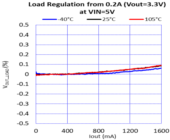
Figure 24. Load Regulation ( V_{IN} = 5.0\text{ V} , V_{OUT} = 3.3\text{ V} )
