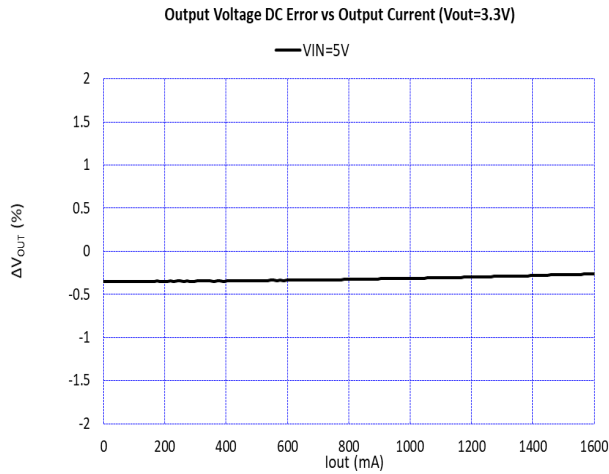
Figure 28. Output Voltage DC Error vs Output Current ( V_{OUT} = 3.3\text{ V} , T_A = 25^\circ\text{C} )
