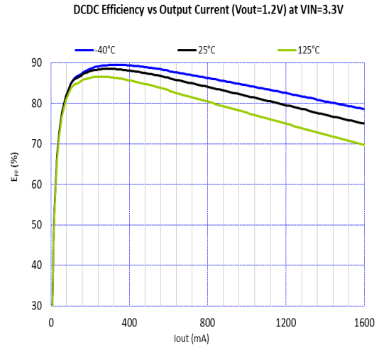
Figure 13. Efficiency vs. Output Current and Temperature at V_{IN} = 3.3\text{ V} ( V_{OUT} = 1.2\text{ V} , L = \text{FDSD0420-H-1R0M} )
