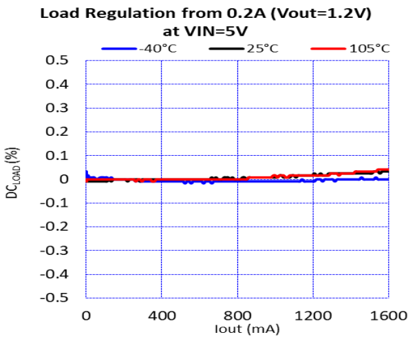
Figure 20. Load Regulation ( V_{IN} = 5.0\text{ V} , V_{OUT} = 1.2\text{ V} )
