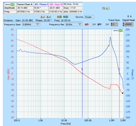
Figure 57. Bode Plot NCV6323FxLMTW18TBG L = 1.0 \mu H - C_{OUT} = 100 \mu F
