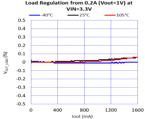
Figure 19. Load Regulation ( V_{IN} = 3.3\text{ V} , V_{OUT} = 1.0\text{ V} )
