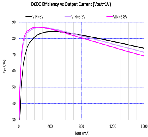
Figure 10. Efficiency vs. Output Current and Input Voltage ( V_{OUT} = 1.0\text{ V} , T_A = 25^\circ\text{C} , L = \text{FDSD0420-H-1R0M} )
