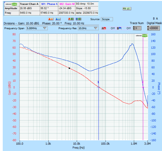
Figure 61. Bode Plot NCV6323FxLMTW12TBG L = 1.0 μH – COUT = 100 μF
