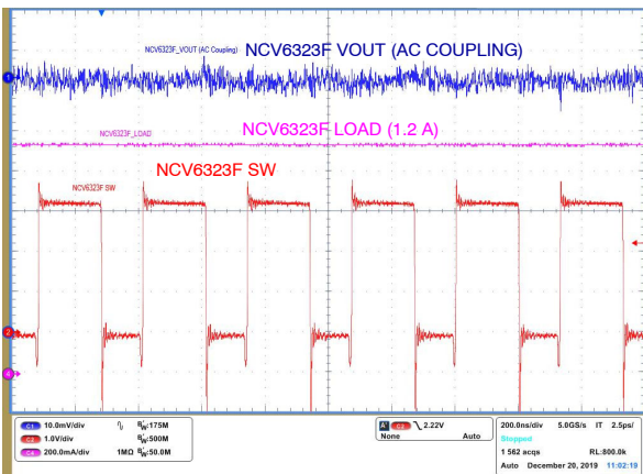
Figure 44. Output Voltage Ripple ( V_{IN} = 3.3\text{ V} , V_{OUT} = 1.8\text{ V} , C_{OUT} = \text{GCM21BR70J106KE22} , I_{OUT} = 500\text{ mA} )
