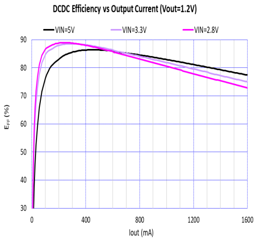
Figure 12. Efficiency vs. Output Current and Input Voltage ( V_{OUT} = 1.2\text{ V} , T_A = 25^\circ\text{C} , L = \text{FDSD0420-H-1R0M} )
