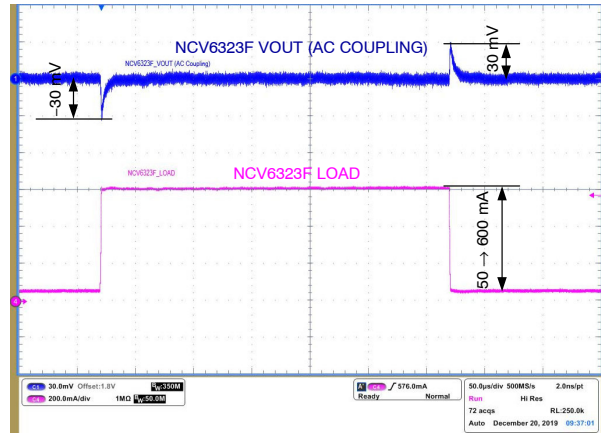
Figure 35. Load Transient ( V_{IN} = 3.3\text{ V} , V_{OUT} = 1.8\text{ V} , C_{OUT} = \text{GCM21BR70J106KE22} , L = \text{FDSD0420-H-1R0M} ) 50 mA \rightarrow 600 mA \rightarrow 50 mA
