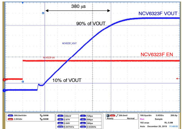
Figure 55. Soft Start Time T_{SS} (NCV6323FELMTW33, C_{OUT} = 10 \mu F )
