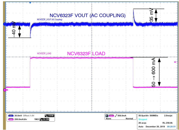
Figure 31. Load Transient ( V_{IN} = 3.3\text{ V} , V_{OUT} = 1.0\text{ V} , C_{OUT} = \text{GCM21BR70J106KE22} , L = \text{FDSD0420-H-1R0M} ) 50 mA \rightarrow 600 mA \rightarrow 50 mA
