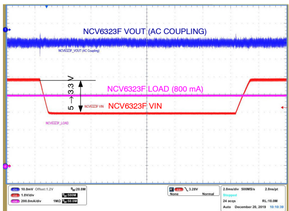
Figure 39. Line Transient ( V_{OUT} = 1.2\text{ V} , C_{OUT} = \text{GCM21BR70J106KE22} , L = \text{FDSD0420-H-1R0M} )
