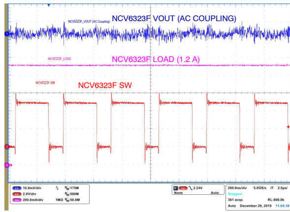
Figure 45. Output Voltage Ripple ( V_{IN} = 5.0\text{ V} , V_{OUT} = 3.3\text{ V} , C_{OUT} = \text{GCM21BR70J106KE22} , I_{OUT} = 500\text{ mA} )
