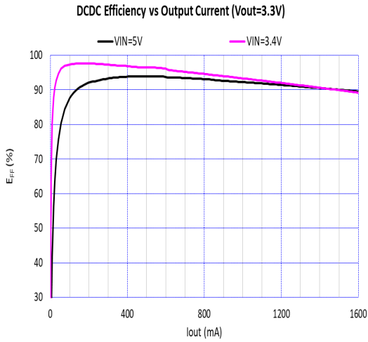
Figure 16. Efficiency vs. Output Current and Input Voltage ( V_{OUT} = 3.3\text{ V} , T_A = 25^\circ\text{C} , L = \text{FSD0420-H-1R0M} )
