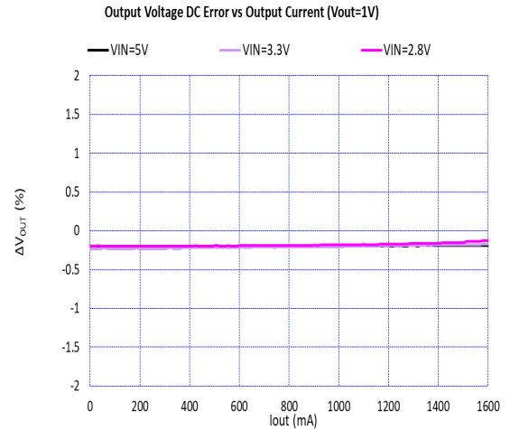
Figure 25. Output Voltage DC Error vs Output Current ( V_{OUT} = 1.0\text{ V} , T_A = 25^\circ\text{C} )
