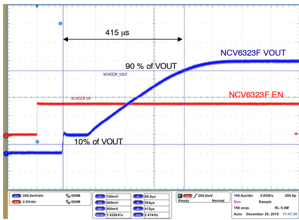
Figure 51. Soft Start Time T_{SS} (NCV6323FELMTW10, C_{OUT} = 10\text{ }\mu\text{F} )
