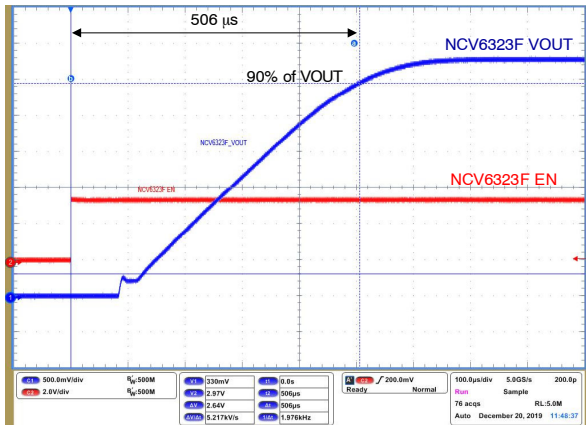
Figure 54. Startup Time T_{START} (NCV6323FELMTW33, C_{OUT} = 10 \mu F )
