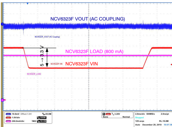
Figure 38. Line Transient ( V_{OUT} = 1.0\text{ V} , C_{OUT} = \text{GCM21BR70J106KE22} , L = \text{FDSD0420-H-1R0M} )
