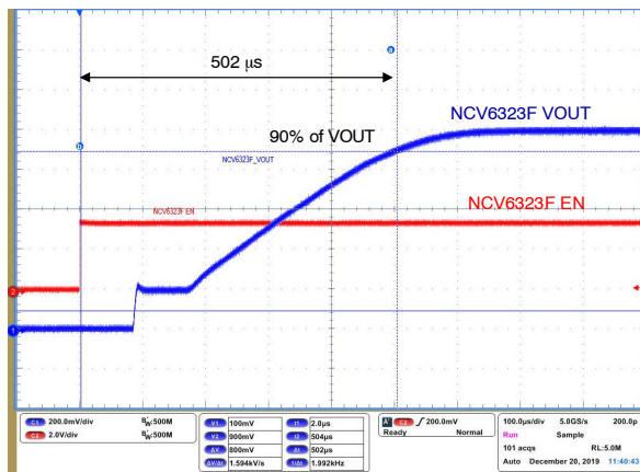
Figure 50. Startup Time T_{START} (NCV6323FELMTW10, C_{OUT} = 10\text{ }\mu\text{F} )
