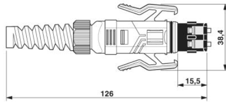
SCRJ plug connector, HCS, IP67
