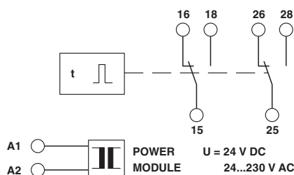
Block diagram
