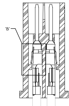
SECTION "A"-A" SCALE 3 : 1
