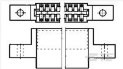
TE Part #583861-5 TW-LEAF CRP HSG. 6 POS. 100 C/
