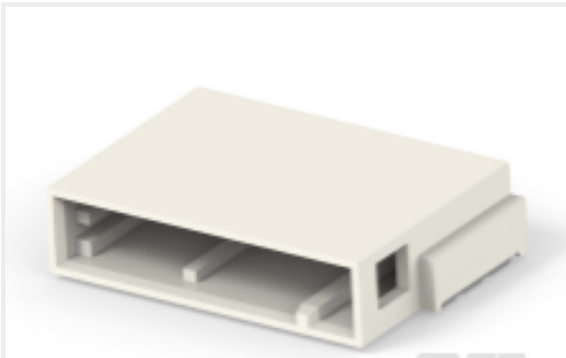
TE Part #2315415-2 10P,TAB0.5X0.4,HDR ASSY,90DEG, COD B
