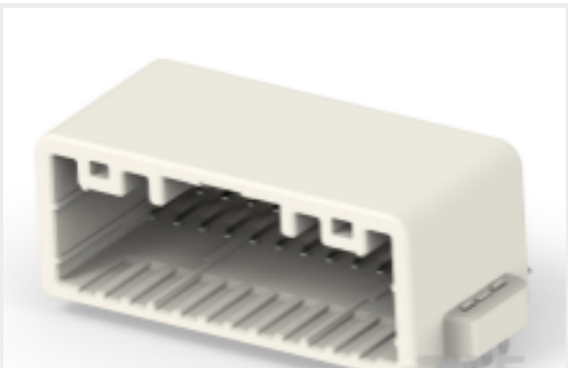
TE Part #2356621-1 24POS,TAB0.64X0.64,HDR ASSY, 90DEG,SMD
