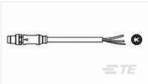
TE Part #1-2273000-1 M8 x 1.0 straight plug Pigtail
