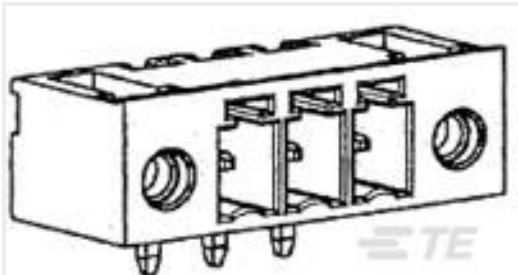
TE Part #796866-3 3 POS TERMI-BLOK HDR RT ANGLE
