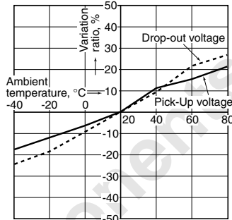
1.-(5) Ambient temperature characteristics (200 A type)
