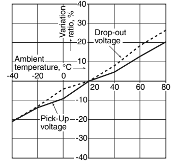
1.-(6) Ambient temperature characteristics (300 A type)
