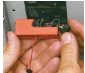
Step 2: Attach the lockout device to the breaker and snap into locked position.
