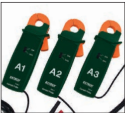
PQ34-2: 200A Current Clamp Probes with 0.8" (19mm) jaw opening
