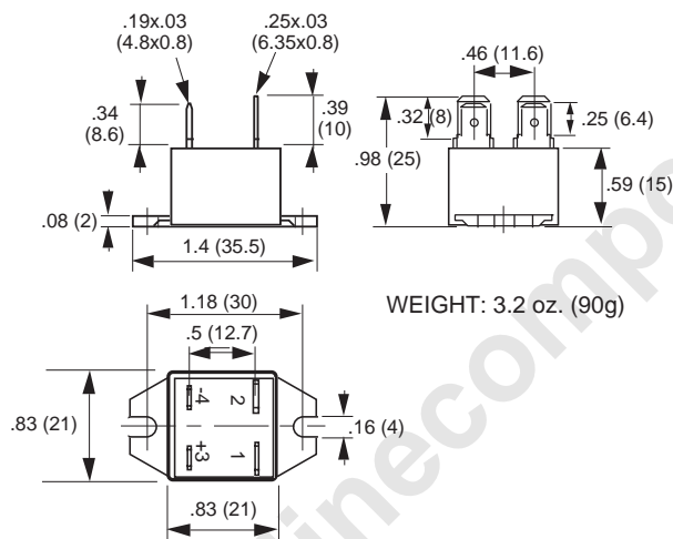
Figure 1a — FS relays except FS24D10
