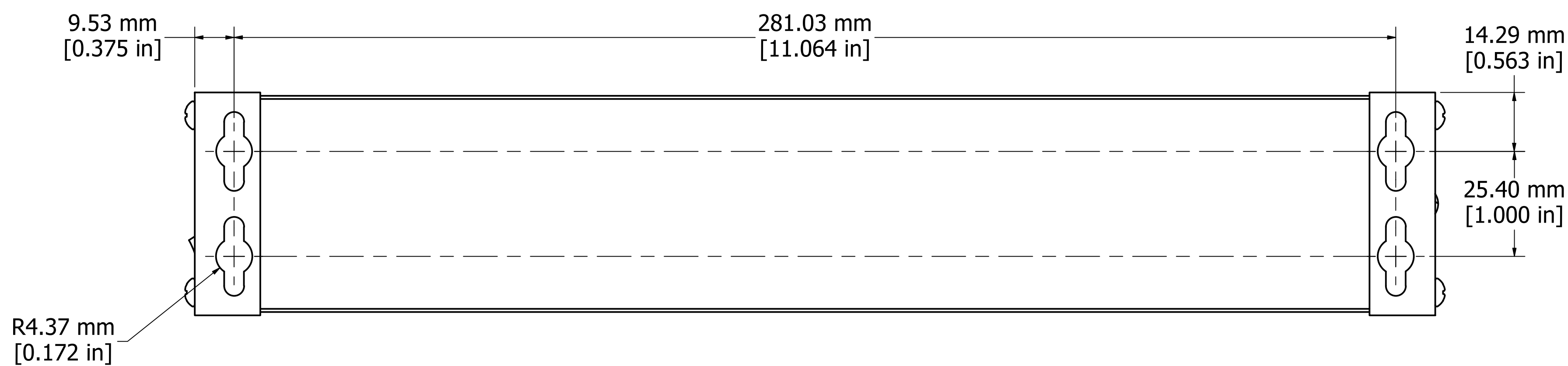
ASSEMBLY - VIEW FROM BOTTOM
