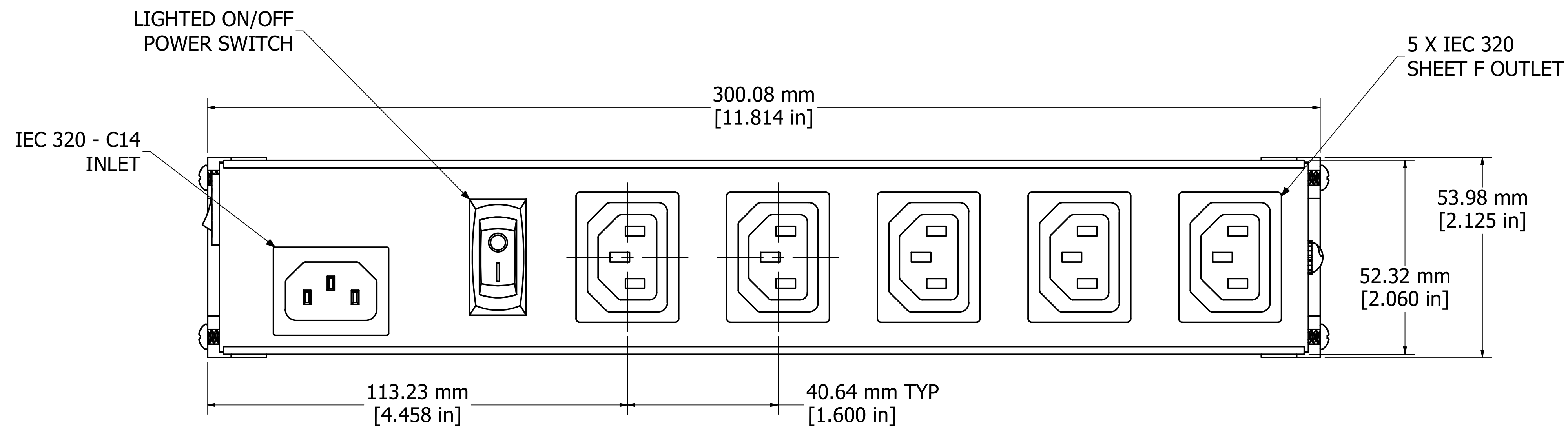
ASSEMBLY - VIEW FROM TOP
