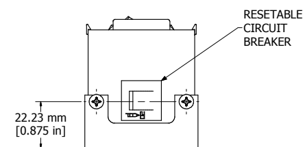
ASSEMBLY - VIEW FROM END
