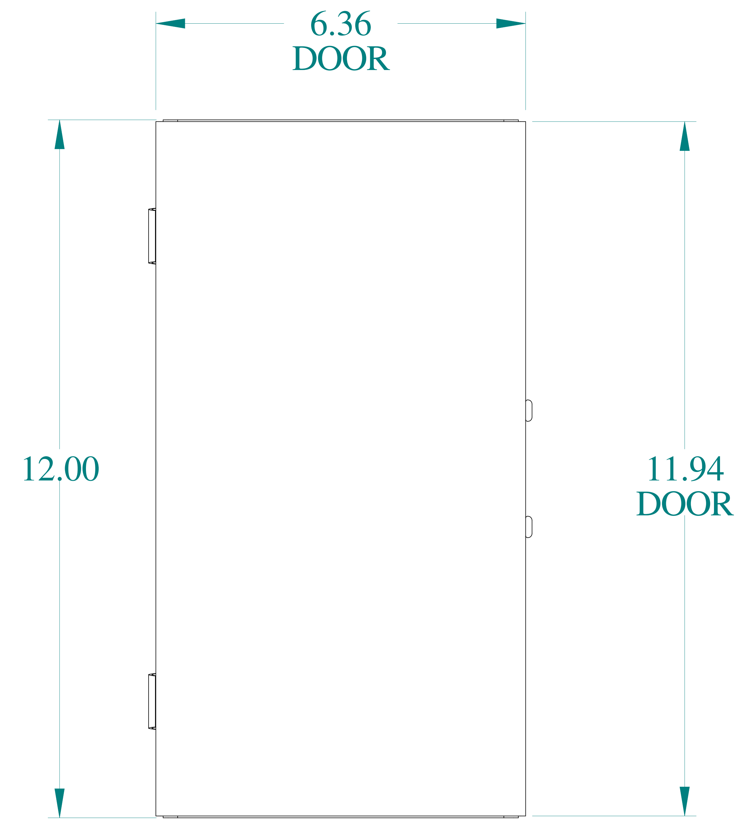
TOP VIEW
