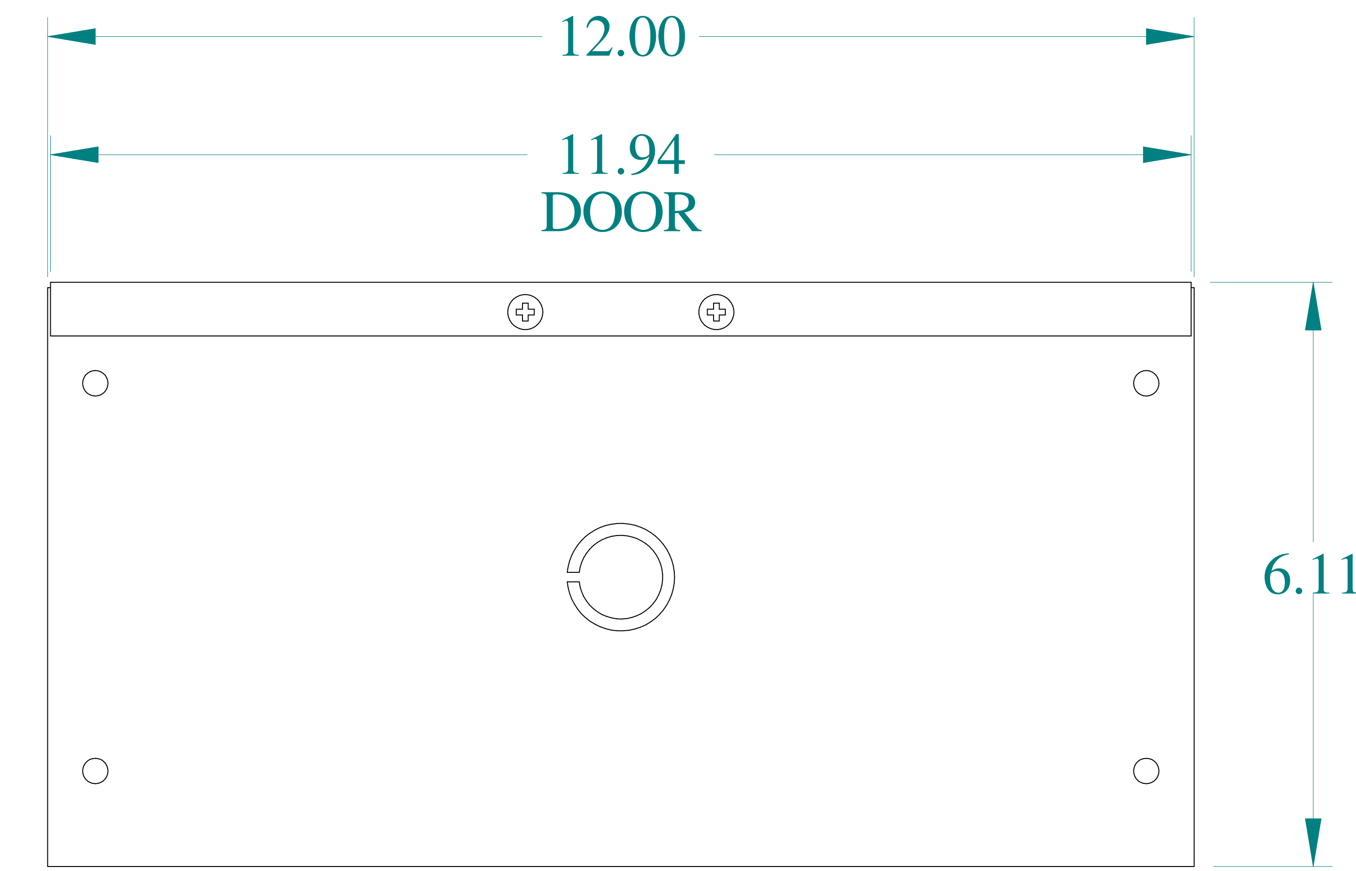
SIDE VIEW
