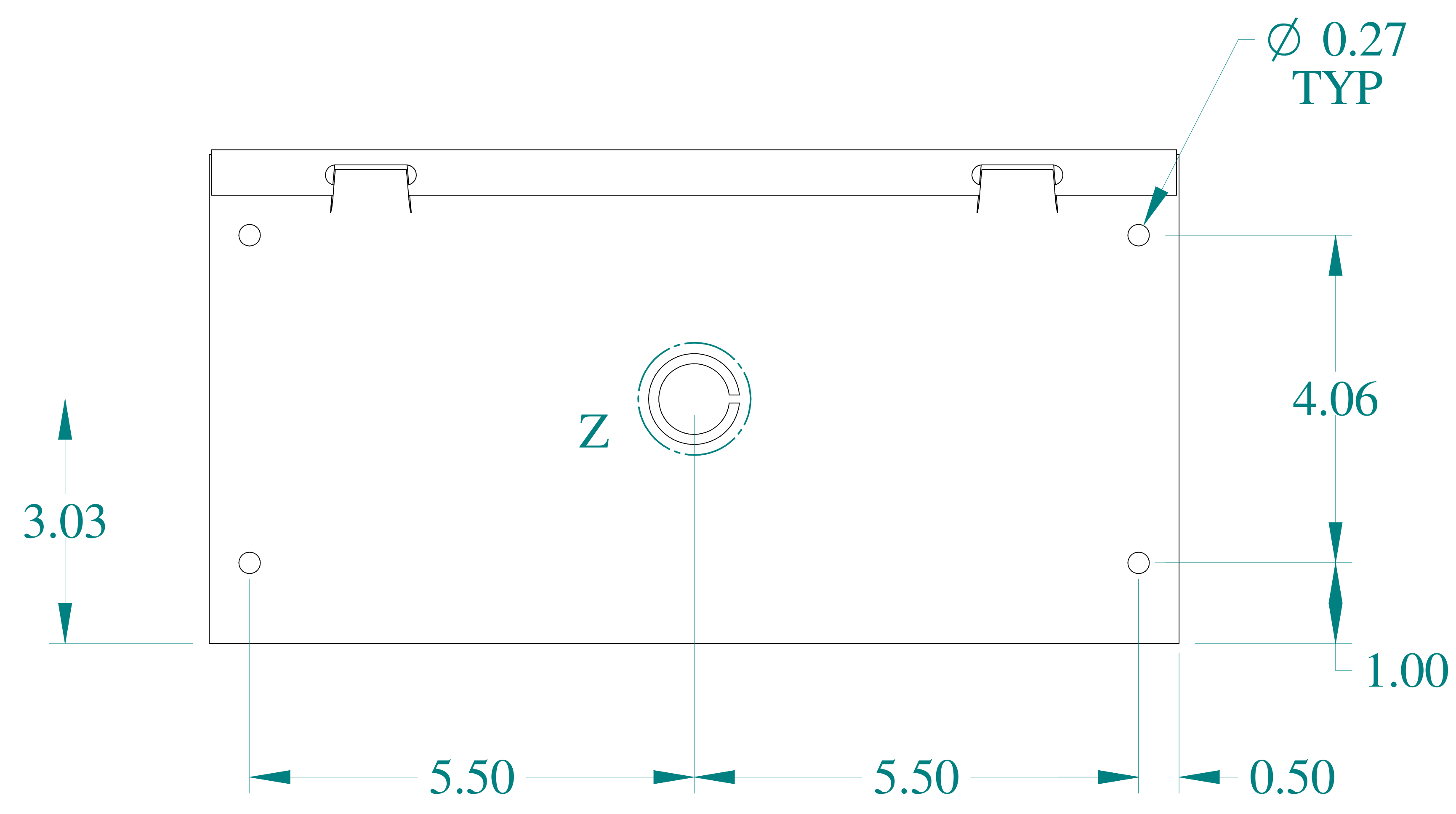
SIDE VIEW
