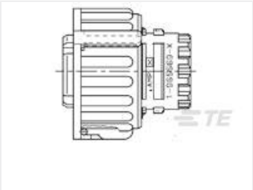
TE Part #1-1813099-1 2.5mm SOCKET HSG ASSEMBLY (BLACK 4 POS)
