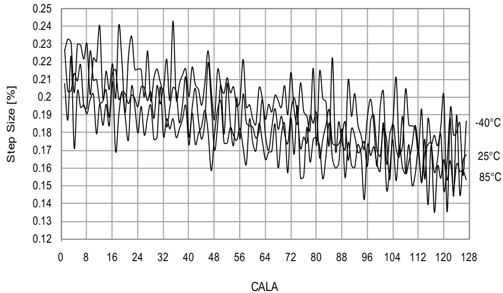
Figure 34-62. 32MHz internal oscillator CALA calibration step size.
