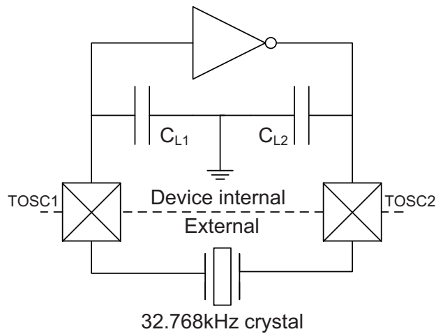
Figure 33-4. TOSC input capacitance.
