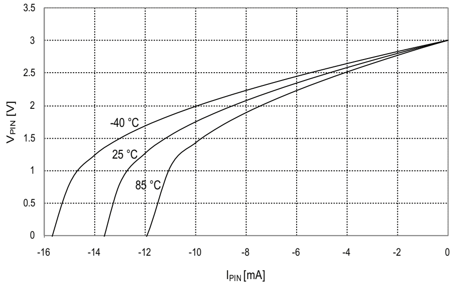
Figure 34-158. I/O pin output voltage vs. source current.
