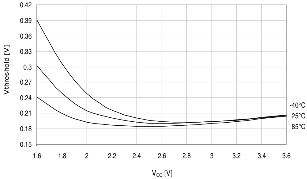
Figure 34-299. I/O pin input hysteresis vs. V_{CC} .
