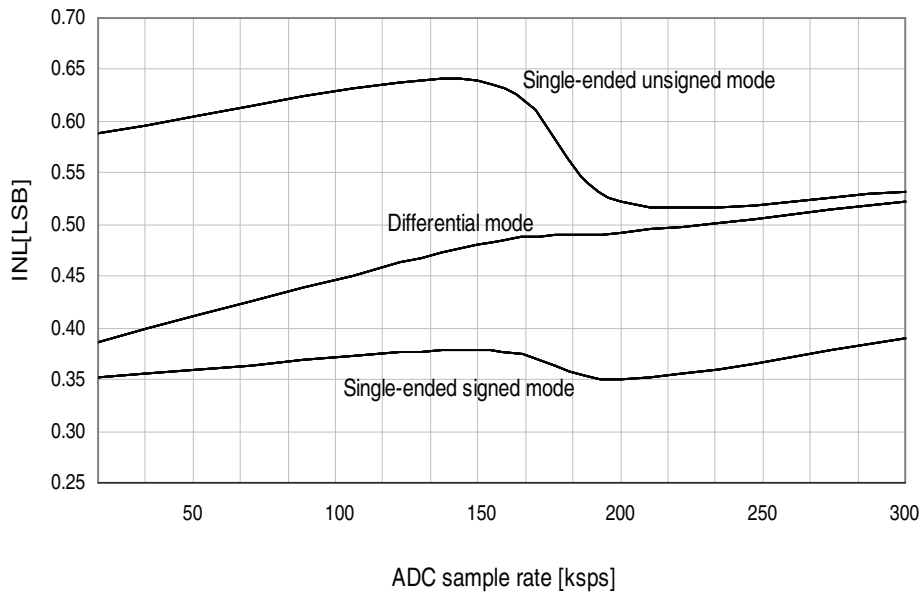
Figure 34-100. INL error vs. sample rate.
