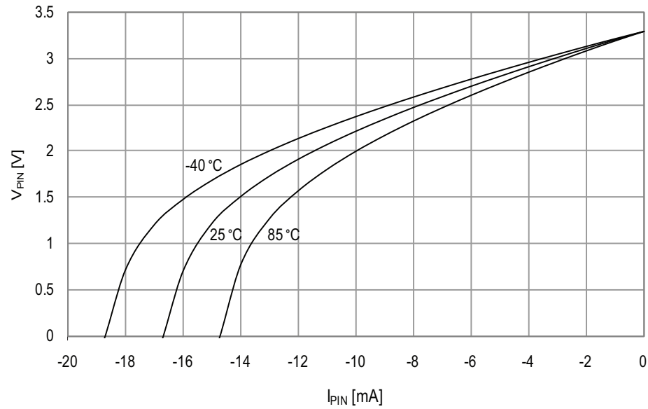
Figure 34-92. I/O pin output voltage vs. source current.
