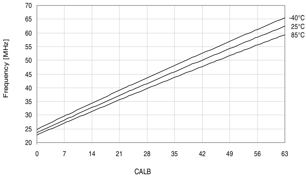
Figure 34-265.32MHz internal oscillator frequency vs. CALB calibration value.
