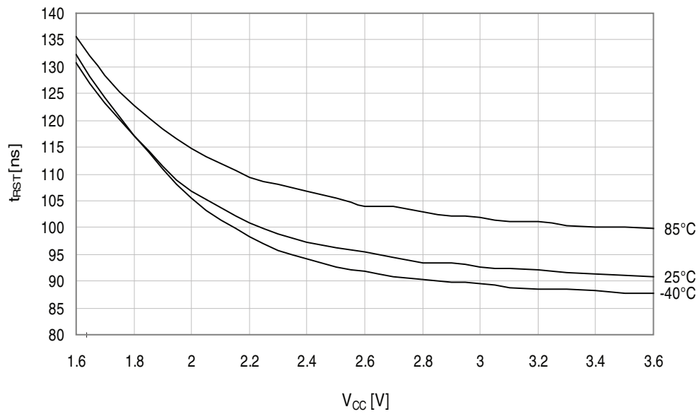
Figure 34-251. Minimum Reset pin pulse width vs. V CC .
