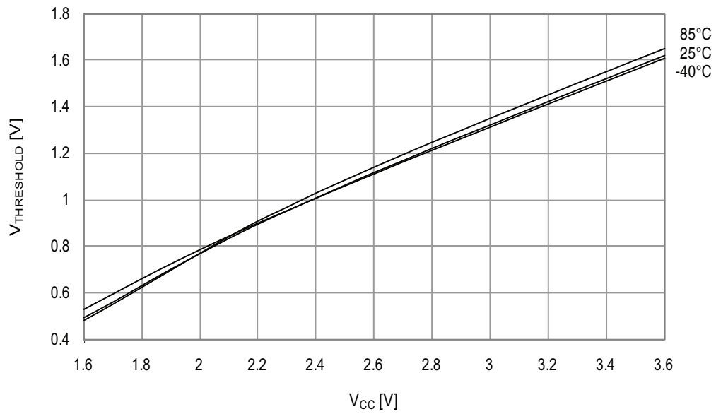
Figure 34-53. Reset pin input threshold voltage vs. V_{CC} .
