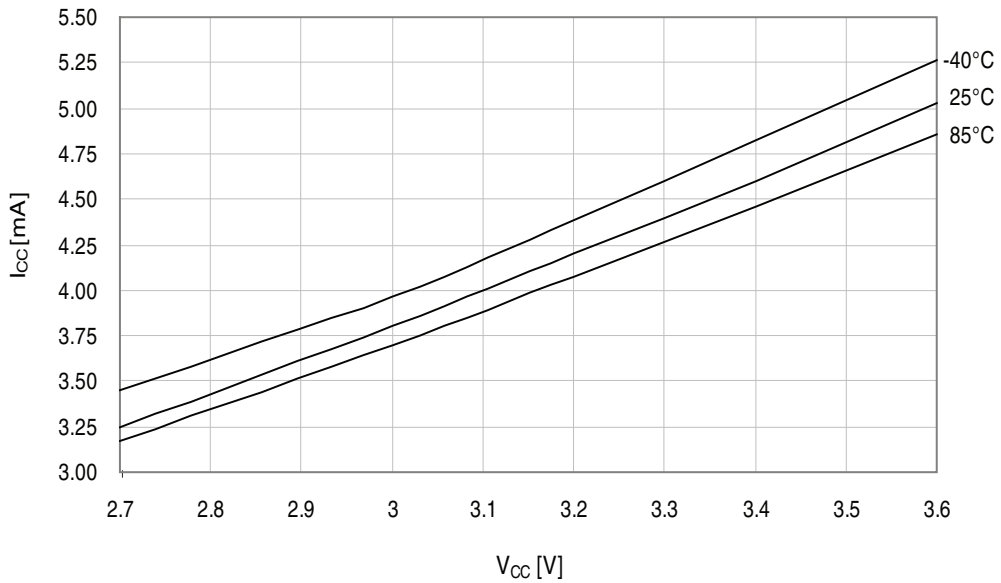
Figure 34-217. Idle mode current vs. V_{CC} .
