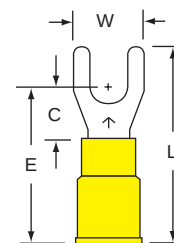
33-10-P Stud Size 10 Wire Range 12-10
