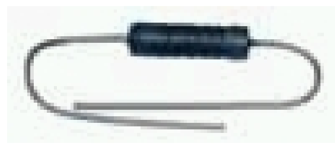
SC Series, 0.5 Ohms, 3.0 W, Fixed, Wirewound Resistor
