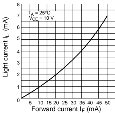
EE-SX1088/1096(-W1)
