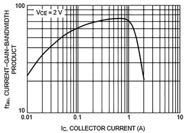
Figure 7. Current-Gain-Bandwidth Product
