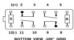
BOTTOM VIEW .100" GRID
