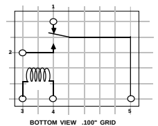
BOTTOM VIEW .100" GRID
