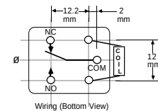
Wiring (Bottom View)
