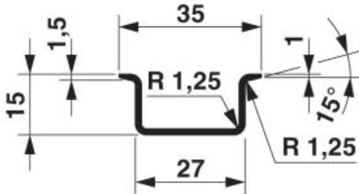
Dimensional drawing
