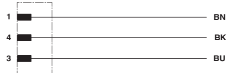
Contact assignment of the M8 plug
