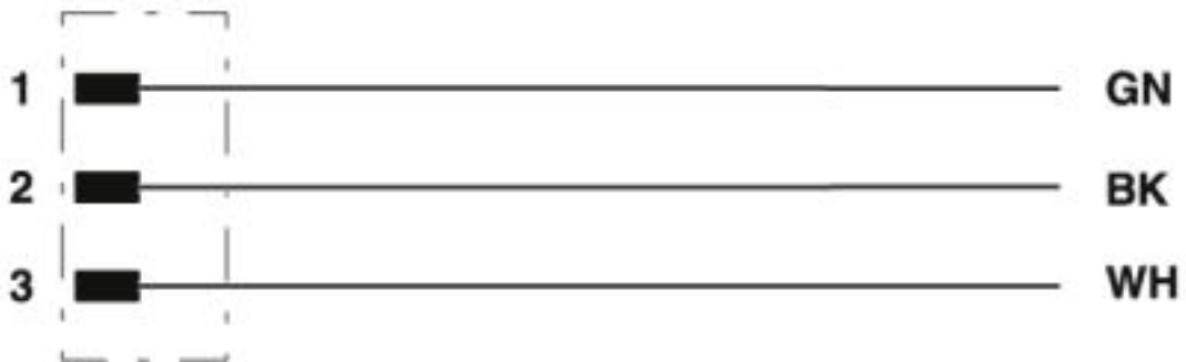
Contact assignment of the 7/8" plug
