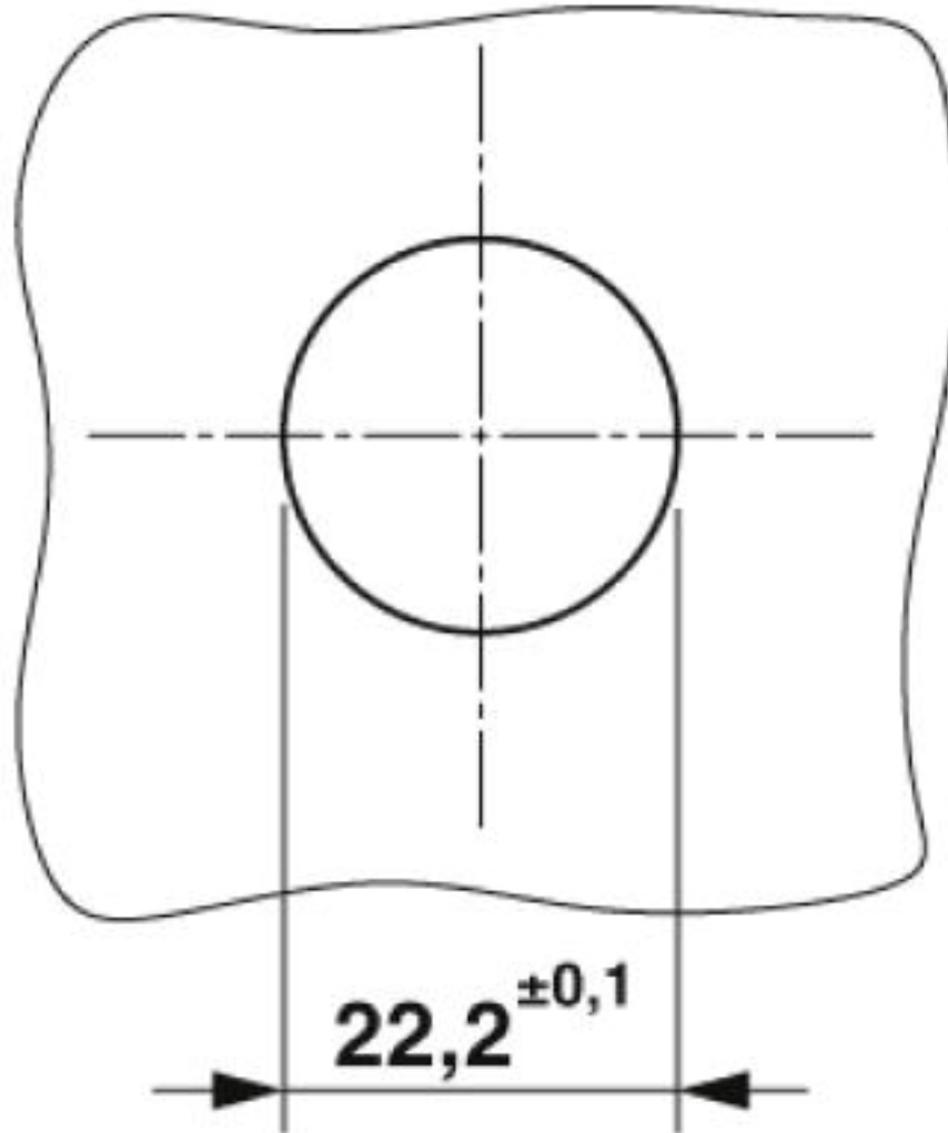
Dimensional drawing
