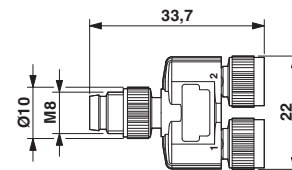
Dimensional drawing
