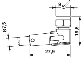
Dimensional drawing
