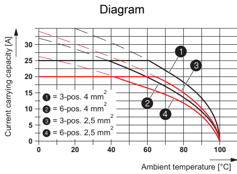
Derating diagram
