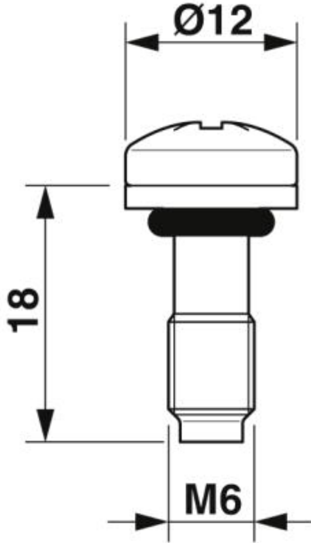
Dimensional drawing
