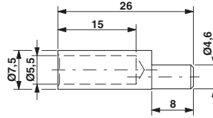
Dimensional drawing
