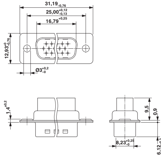
Dimensional drawing
