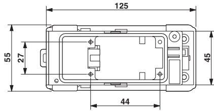
Dimensional drawing
