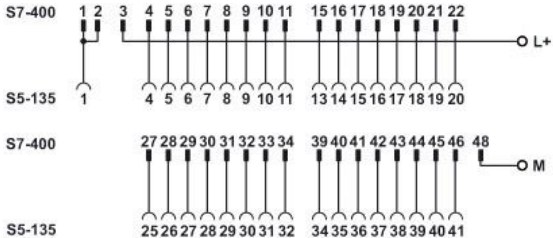
Connection scheme: FLKM S135/S400/SO120
