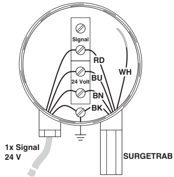
Circuit diagram
