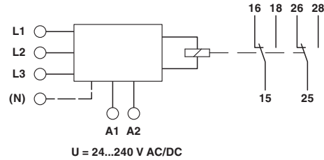
Block diagram
