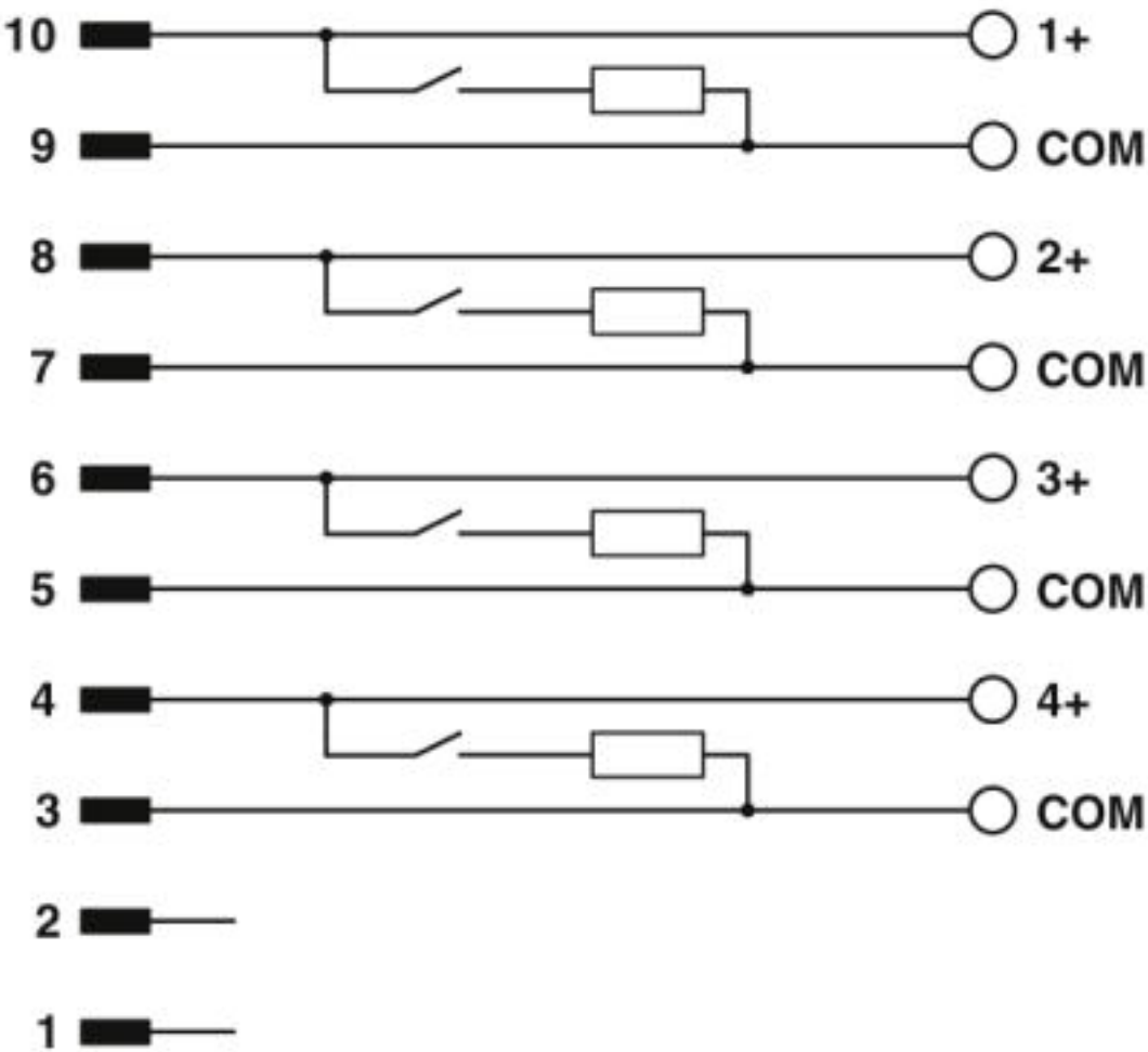
Circuit diagram
