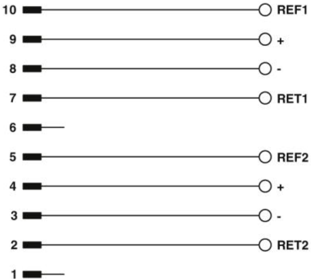
Connection scheme VIP-2/.../FLK50 (1-40) /S7
