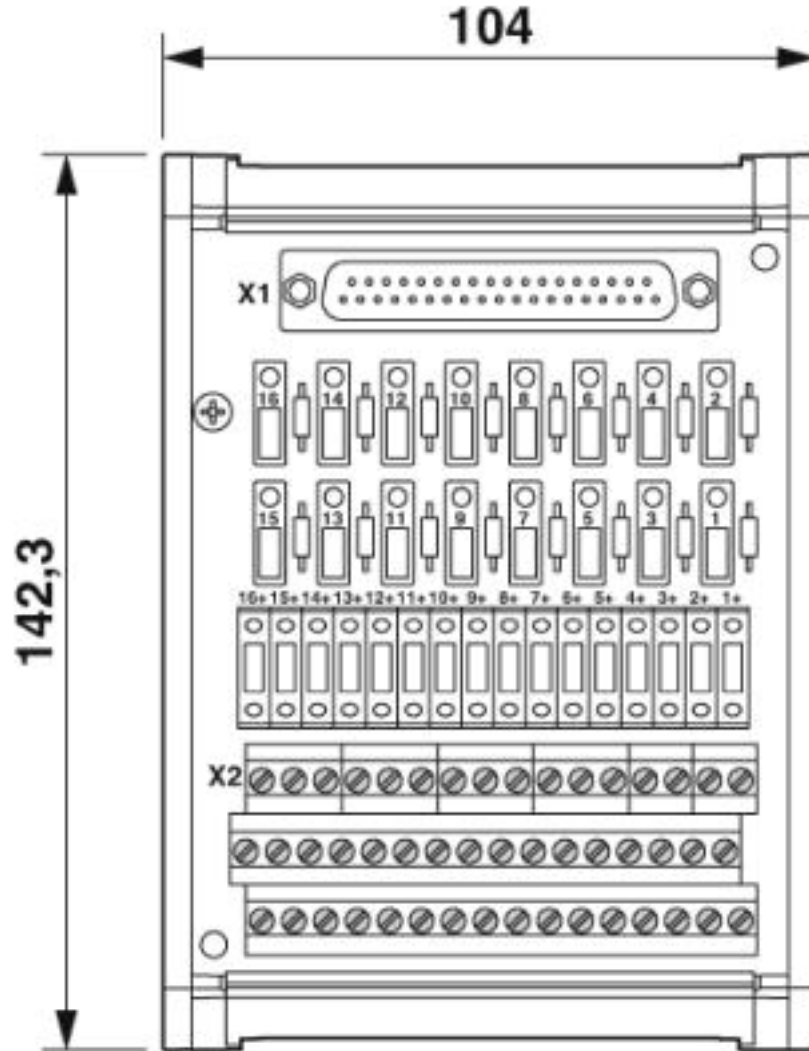
Dimensional drawing
