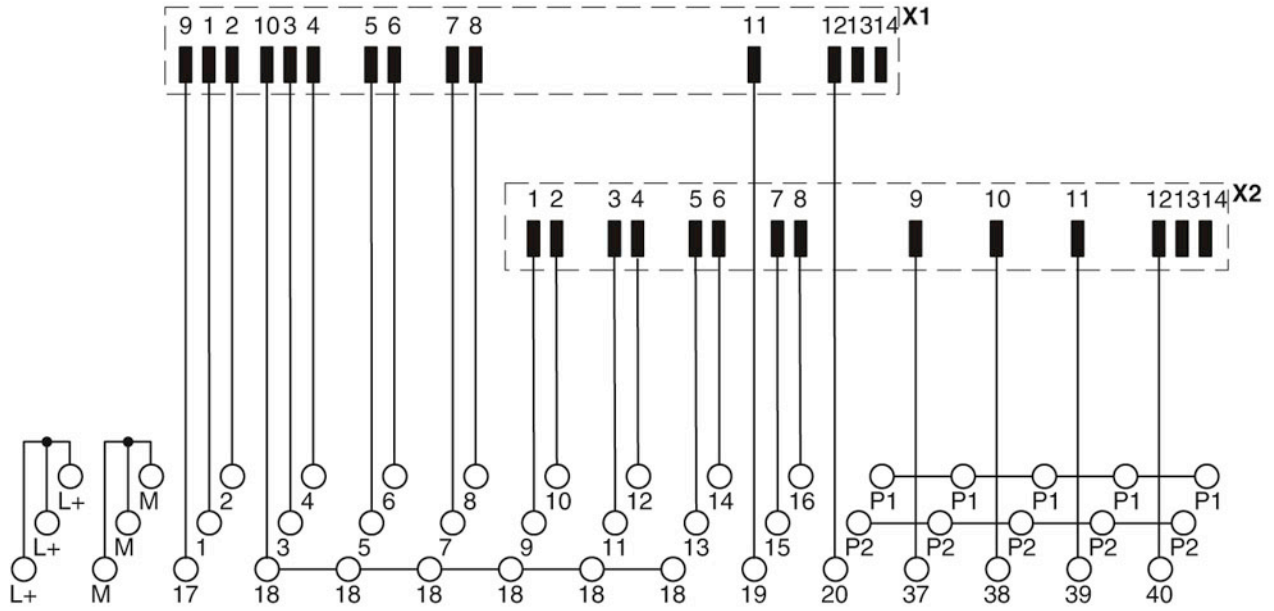
Circuit diagram
