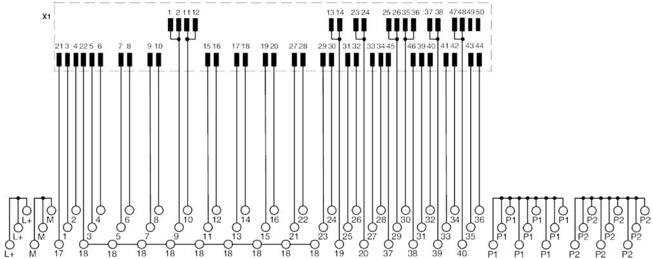
Circuit diagram
