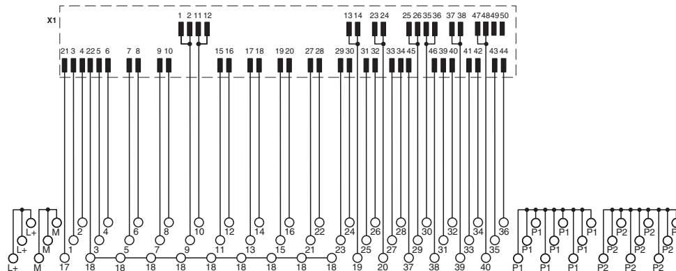
Circuit diagram
