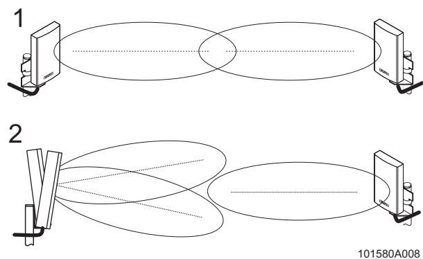
Figure 35 Correct transmitter and receiver beam (1); transmitter and receiver beam outside the target area (2)
