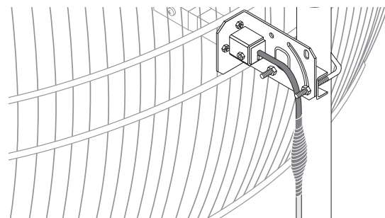
Figure 54 Cable protected
