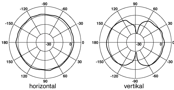
Figure 8 Directional characteristics of the omnidirectional antenna
