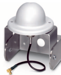
Figure 17 RAD-ISM-2400-ANT-VAN-3-1-MCX omnidirectional antenna
