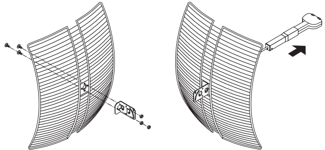
Figure 48 Horizontal polarization
