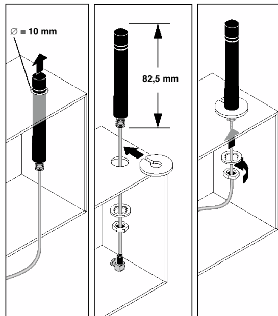
Figure 11 Hole mounting
