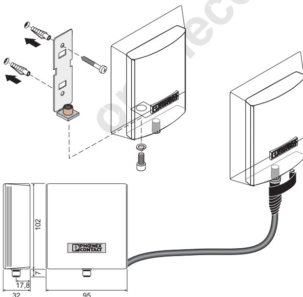
Figure 41 Wall mounting
