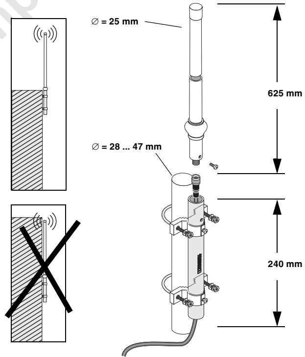
Figure 32 Hole mounting
