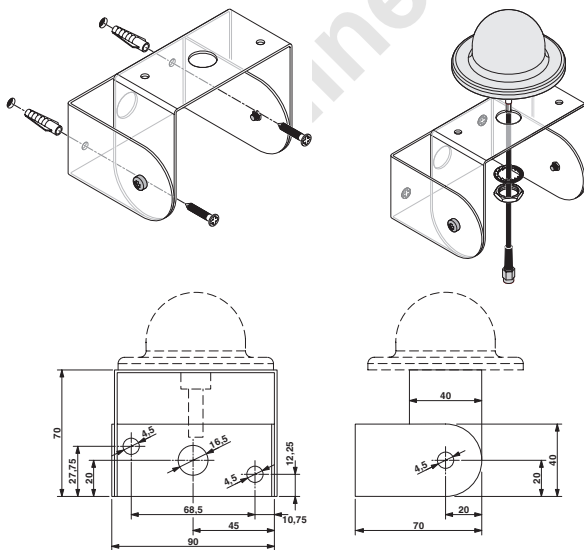
Figure 16 Wall mounting with bracket
