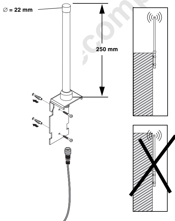
Figure 26 Wall mounting
