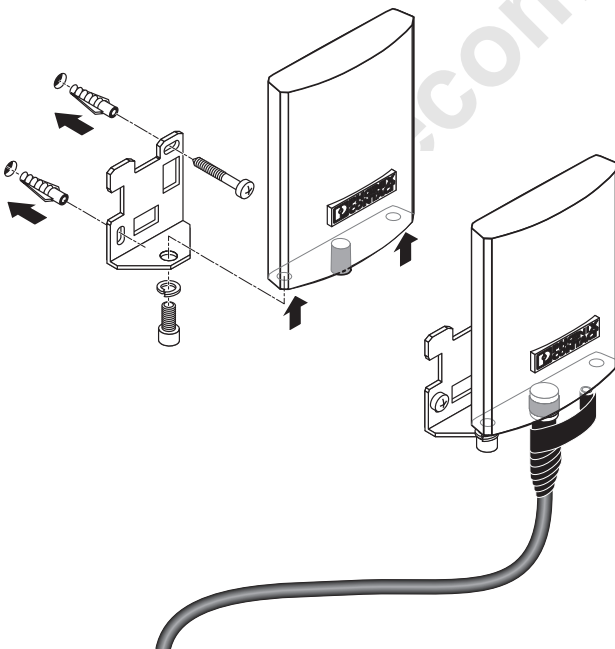
Figure 37 Wall mounting
