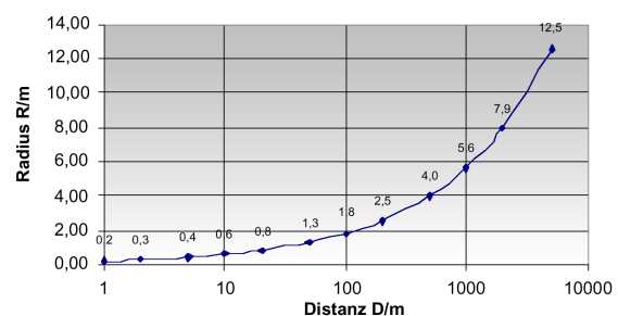
Figure 4 Radius R of the Fresnel zone over distance D
