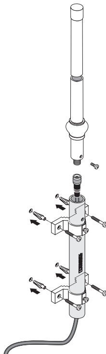
Figure 30 Wall mounting
