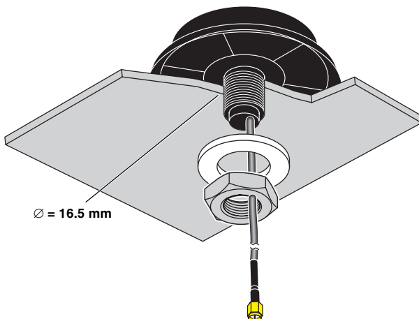
Figure 57 Mounting
