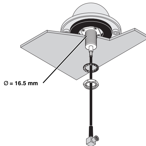
Figure 18 Cabinet mounting
